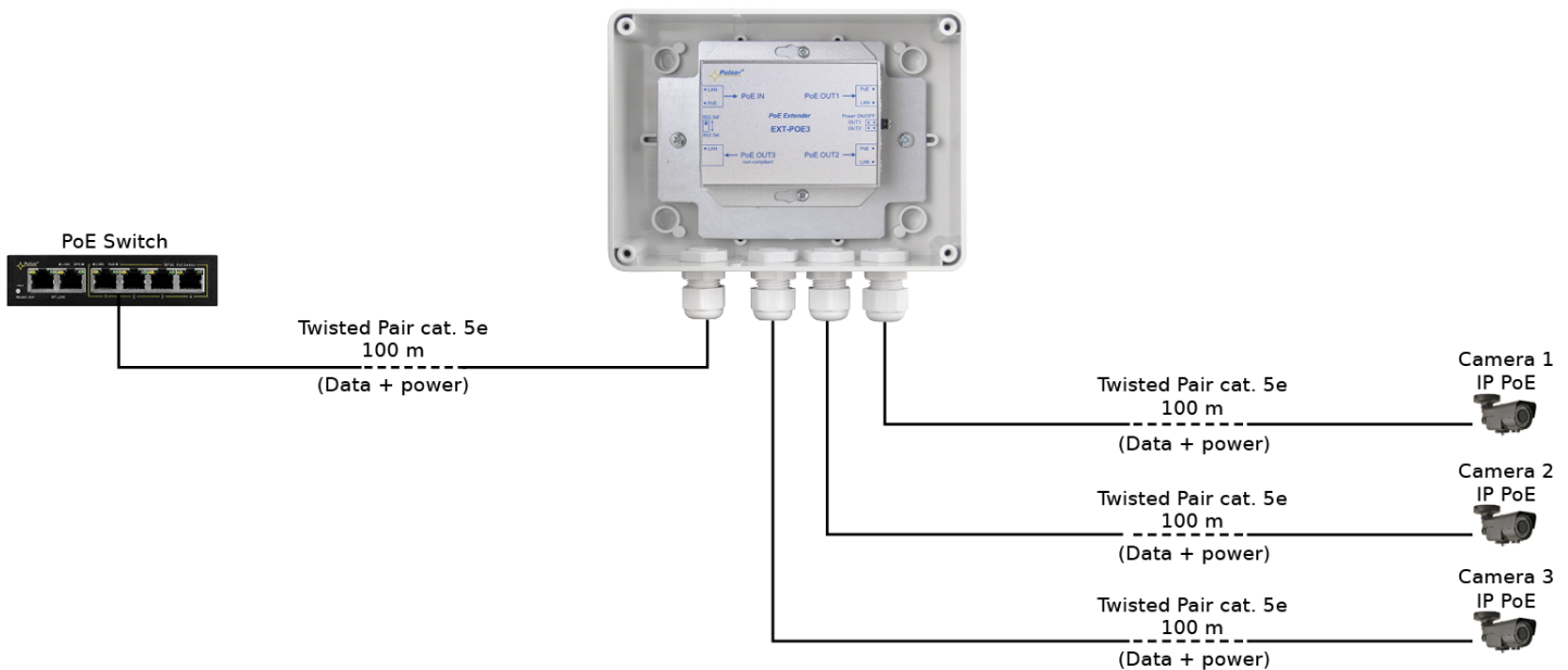
Connection of three IP PoE cameras and extension of the range for another 100m
